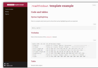
Figure 13.16.: Modèle readthedown
