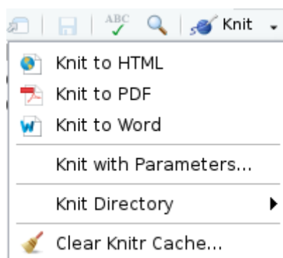
Figure 13.11.: Menu Knit
