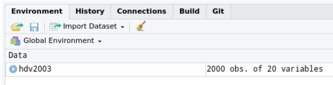
Figure 3.1.: Onglet Environment
